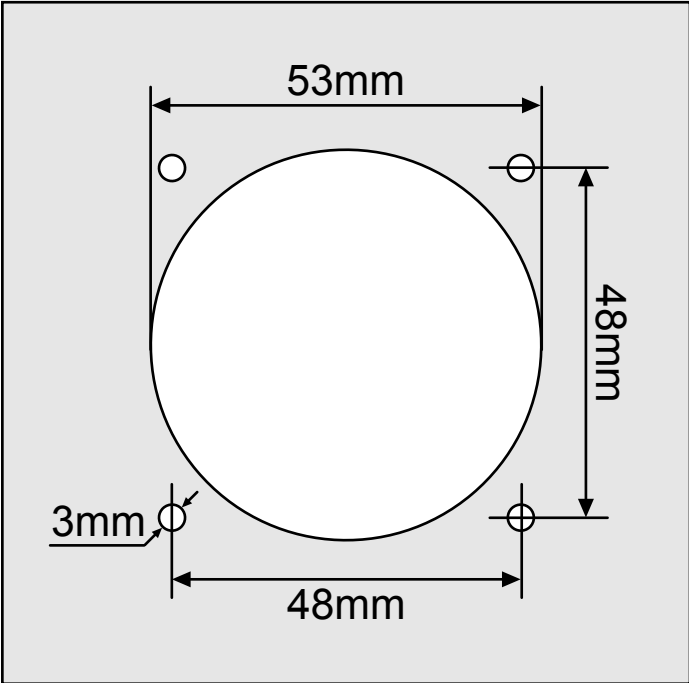
Panel Cutout
